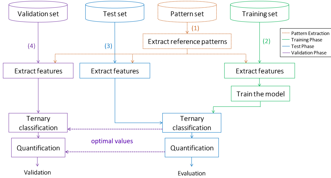
Figure 5.8: Flowchart of the Proposed Approach
