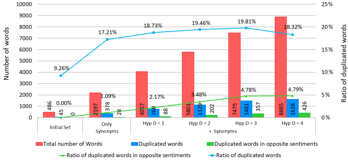
Figure 3.21: Number of Unigrams Collected from WordNet Using the Seed Words Proposed
