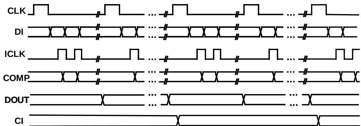
Figure 4.1 Architecture of ADC with Calibration.
