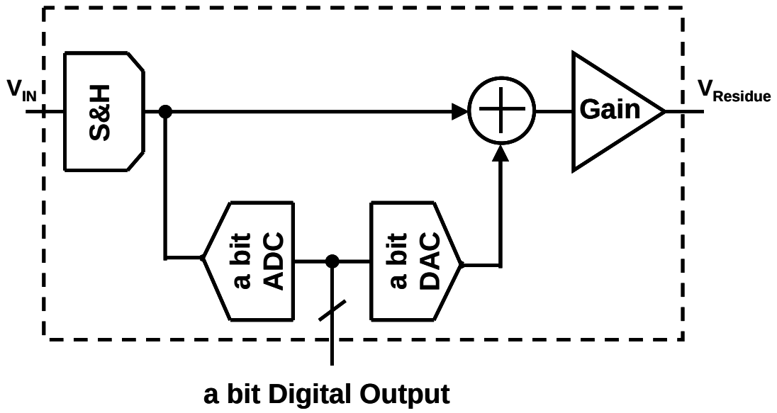
(b) MDAC
