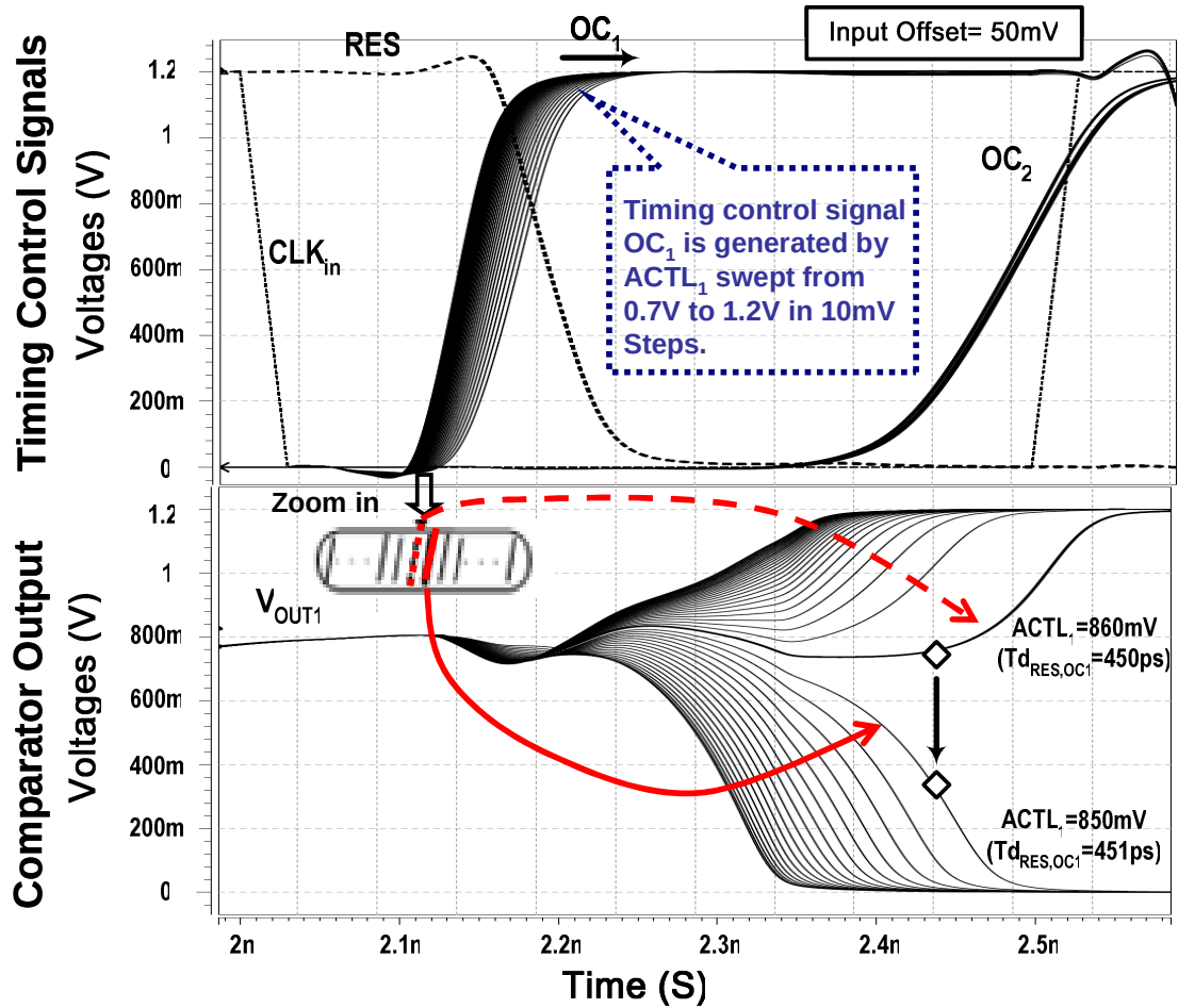
Figure 3.8 Simulation results.
