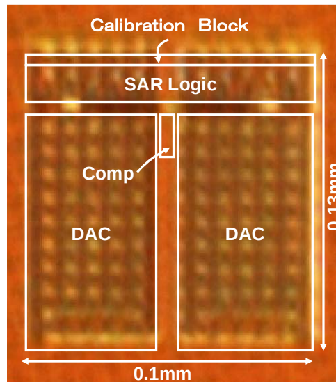
Figure 4.10 Chip photograph.
