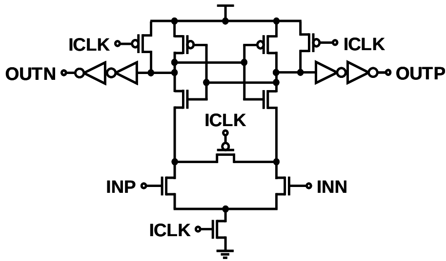
Figure 4.8 Comparator.
