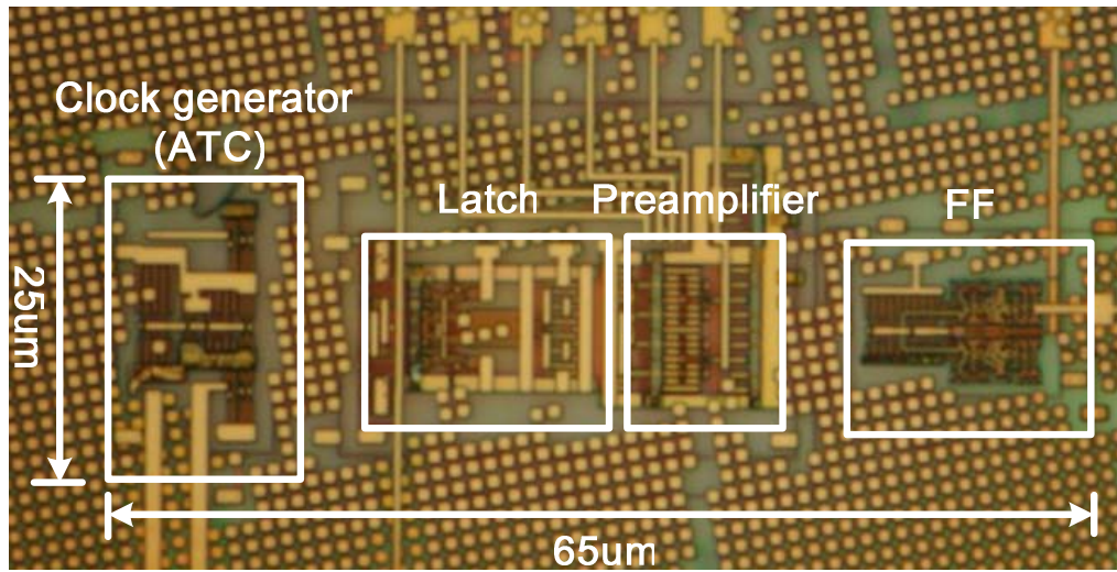
Figure 3.10 Photograph of the comparator test die.
