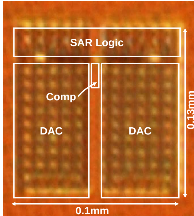
Figure 5.4 Chip photograph.
