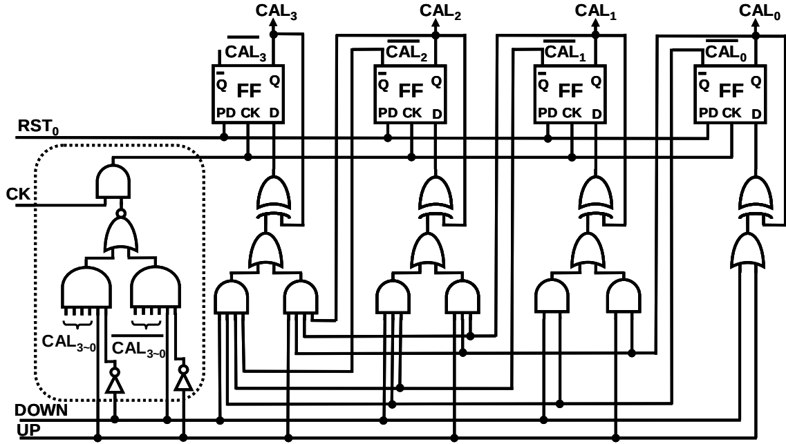
Figure 4.7 Circuits diagram of down/up counter.
