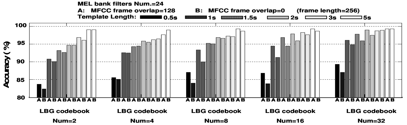
Figure 4.6 Average Recognition Accuracy as a Function of the Template Length and LBG Codebook Cluster Number k .
