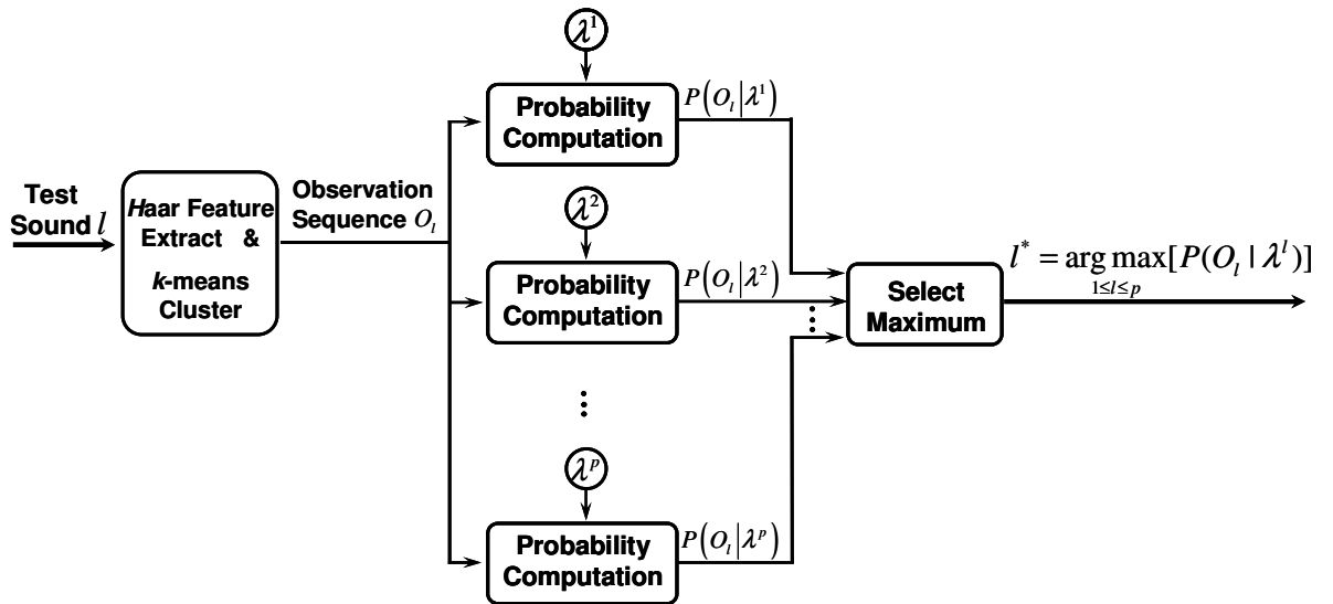
Figure 5.4 Block Diagram of a Test Sound's HMM Classification.
