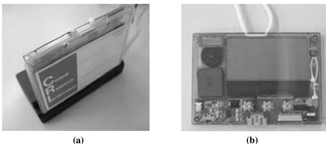
Figure 2.1 Wearable Sensor Recharging on a Charging Pad (a) and Inner Hardware Prototype (b).
