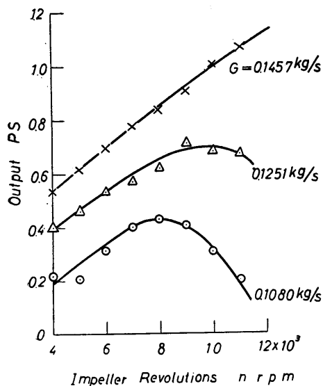
Fig. 15. Relation between output and n ( z=16 )
