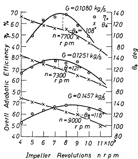
Fig. 10. Relation between \eta_0 and \theta_e ( z=16 )
