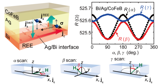
図2. Rashba-Edelstein magnetoresistance.
