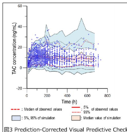
図3 Prediction-Corrected Visual Predictive Check
