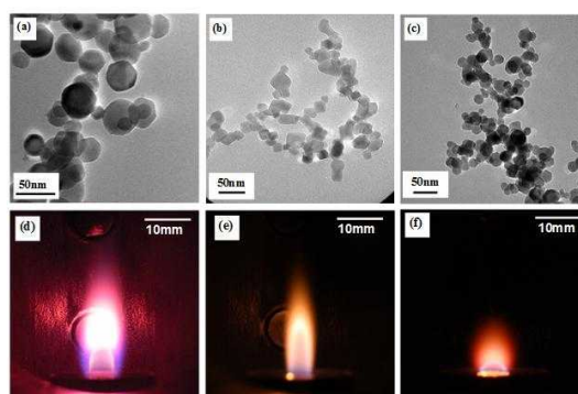
Fig. 2 TEM images of phosphors and flames; (a)(d) T_{ad}=3056\text{K} , p=100\text{kPa} , (b)(e) T_{ad}=2643\text{K} , p=100\text{kPa} , (c)(f) T_{ad}=2891\text{K} , p=25\text{kPa} .
