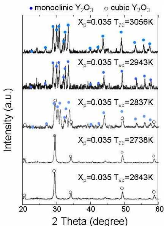
Fig. 5 XRD patterns for various flame temperatures.
