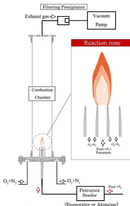
Fig. 1 Experimental apparatus.
