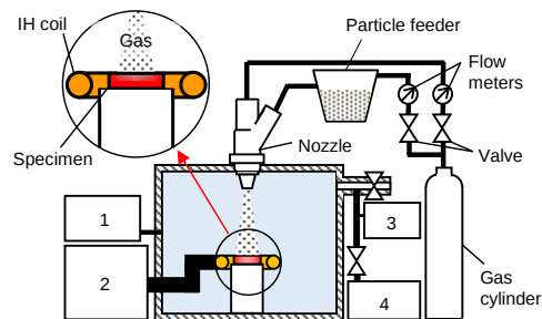
Fig. 1 Experimental apparatus (Legend: 1. vacuum gauge, 2. induction heating inverter, 3. oxygen analyzer, 4. vacuum pump).
