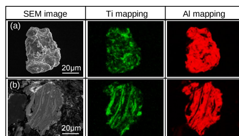
Fig.1 SEM image and EDX mapping of Ti/Al MM particles. (a)appearance and (b)cross section.
