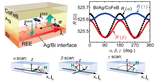
図2. Rashba-Edelstein magnetoresistance.
