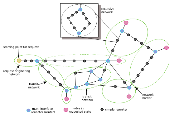
図 9 Quantum Recursive Network Architecture
