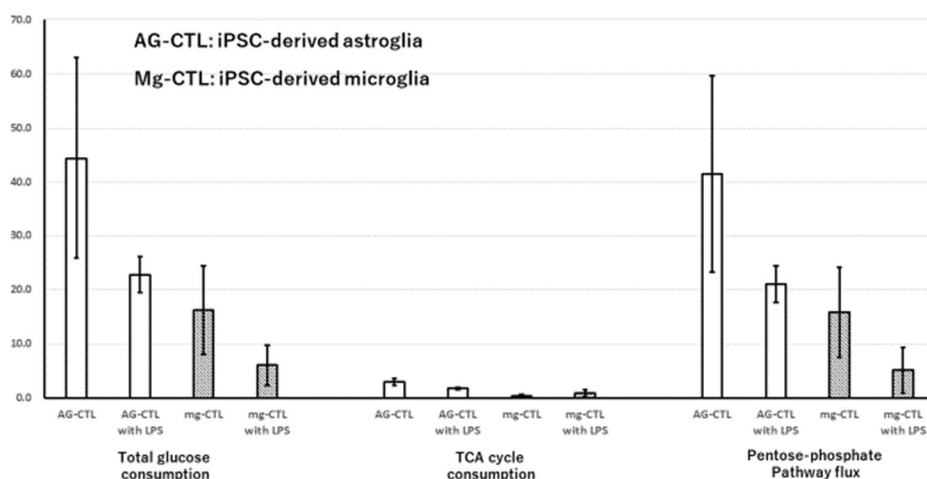
Fig. 2 Characterization of glucose metabolism in human iPSC-derived astroglia and microglia (healthy adults) with and without LPS
