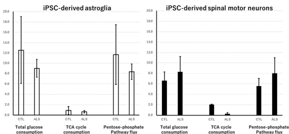
Fig. 1 Characterization of glucose metabolism in human iPSC-derived astroglia and spinal motor neurons (healthy adults vs. ALS patients)
