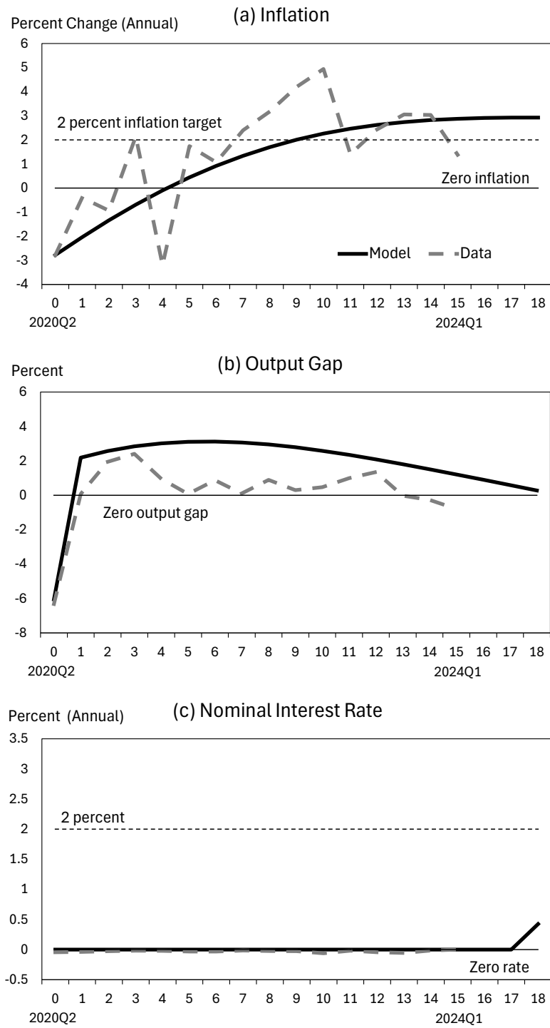
Figure 9: Simulation for Japanese Monetary Policy: Low State Economy
