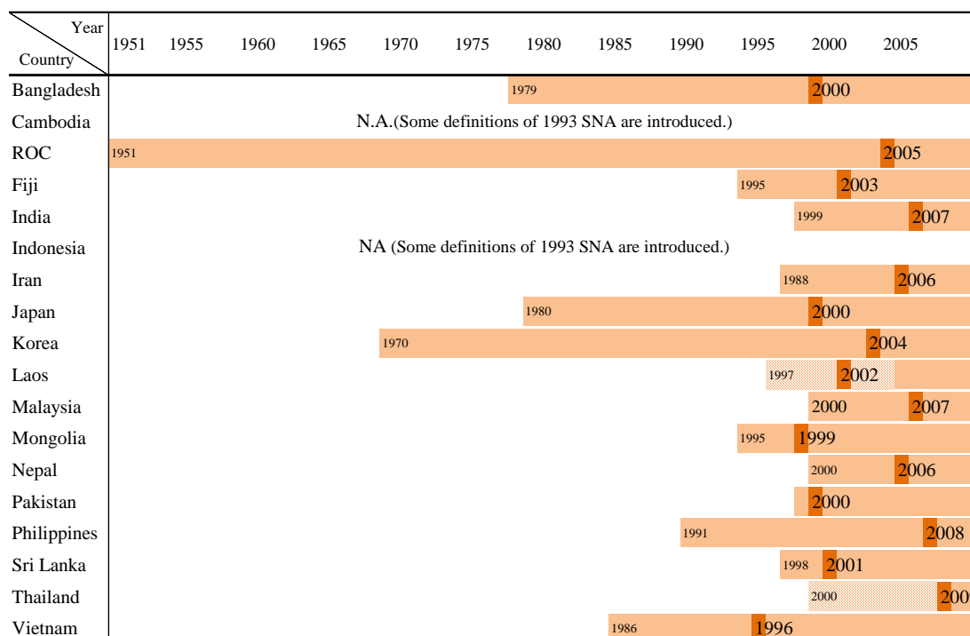
Figure 2: Implementation of 1993 SNA
